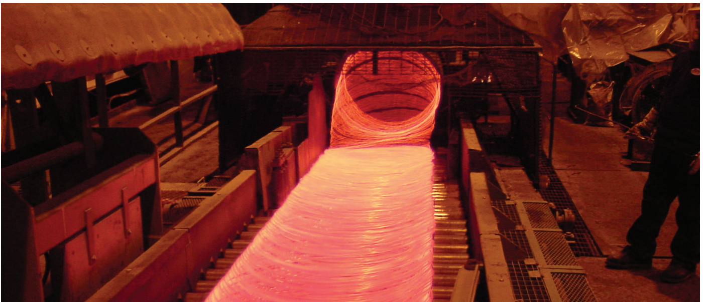
At its facility in Sterling, IL, Leggett & Platt shuts down the coiled steel rod cooling operation during DR dispatches.
